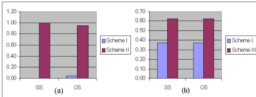
Figure 1: Hard decision Subjective and Objective performance assessment with L=1.5 , \Gamma_g=0.9994 , \kappa_g=15 , \sigma_g=0.5 and \Gamma_\alpha=0.9879 , \kappa_\alpha=22 , \sigma_\alpha=0.8
